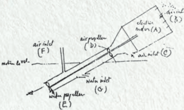
Chraipattana Aerator Model X 5
